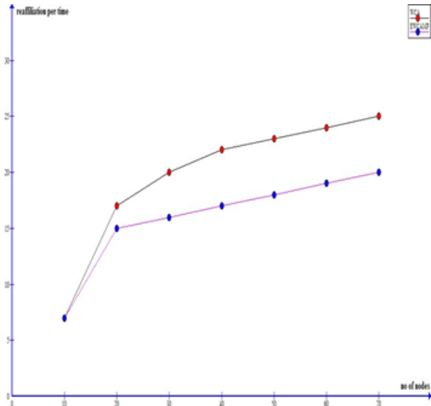
Figure 5: Average re-affiliation frequency vs node number
